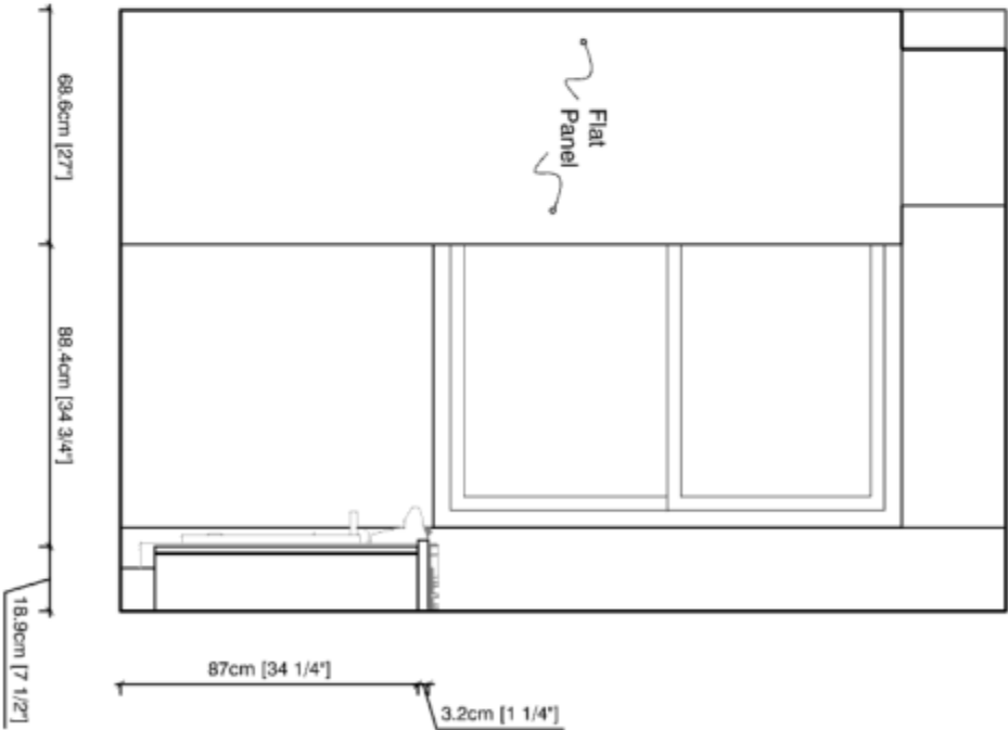
ELEVATION-"C"
