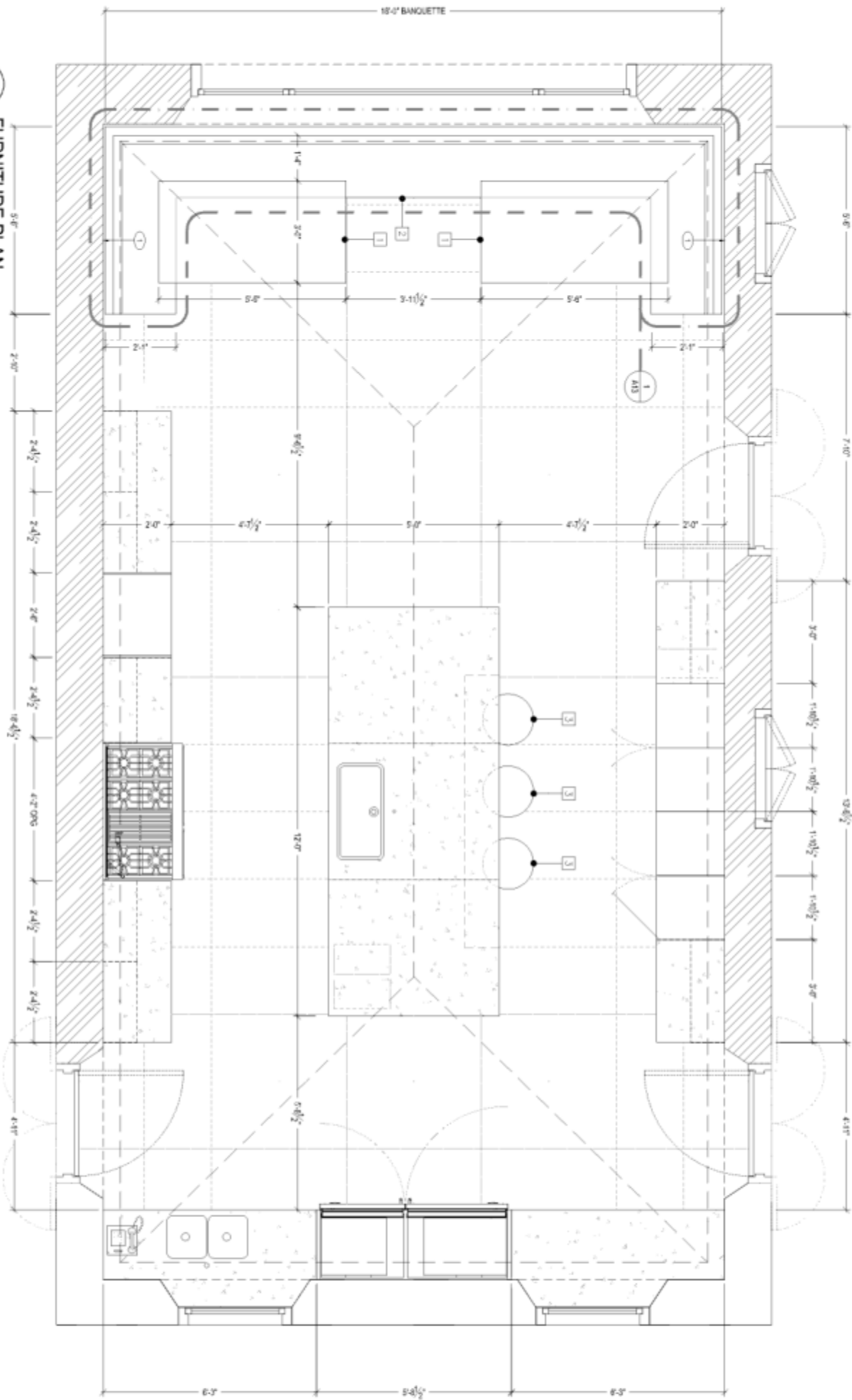
1 FURNITURE PLAN SCALE: 1/2"=1'-0"
