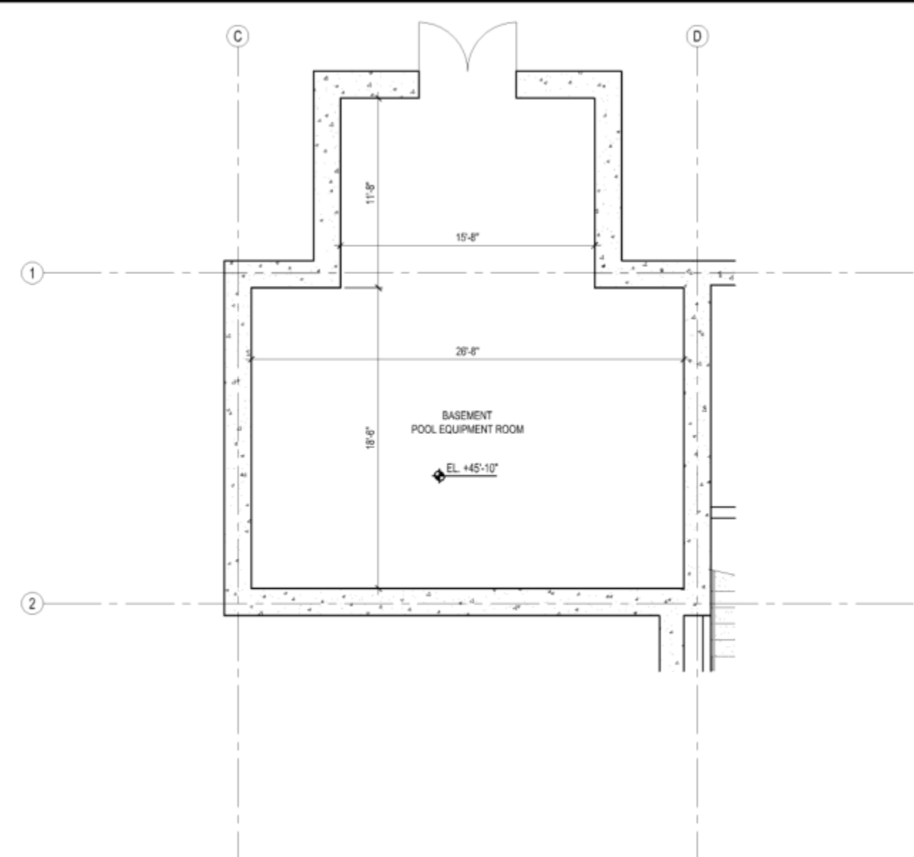
ENLARGED PLAN - POOL EQUIPMENT ROOM SCALE: 1/4" = 1'-0"
