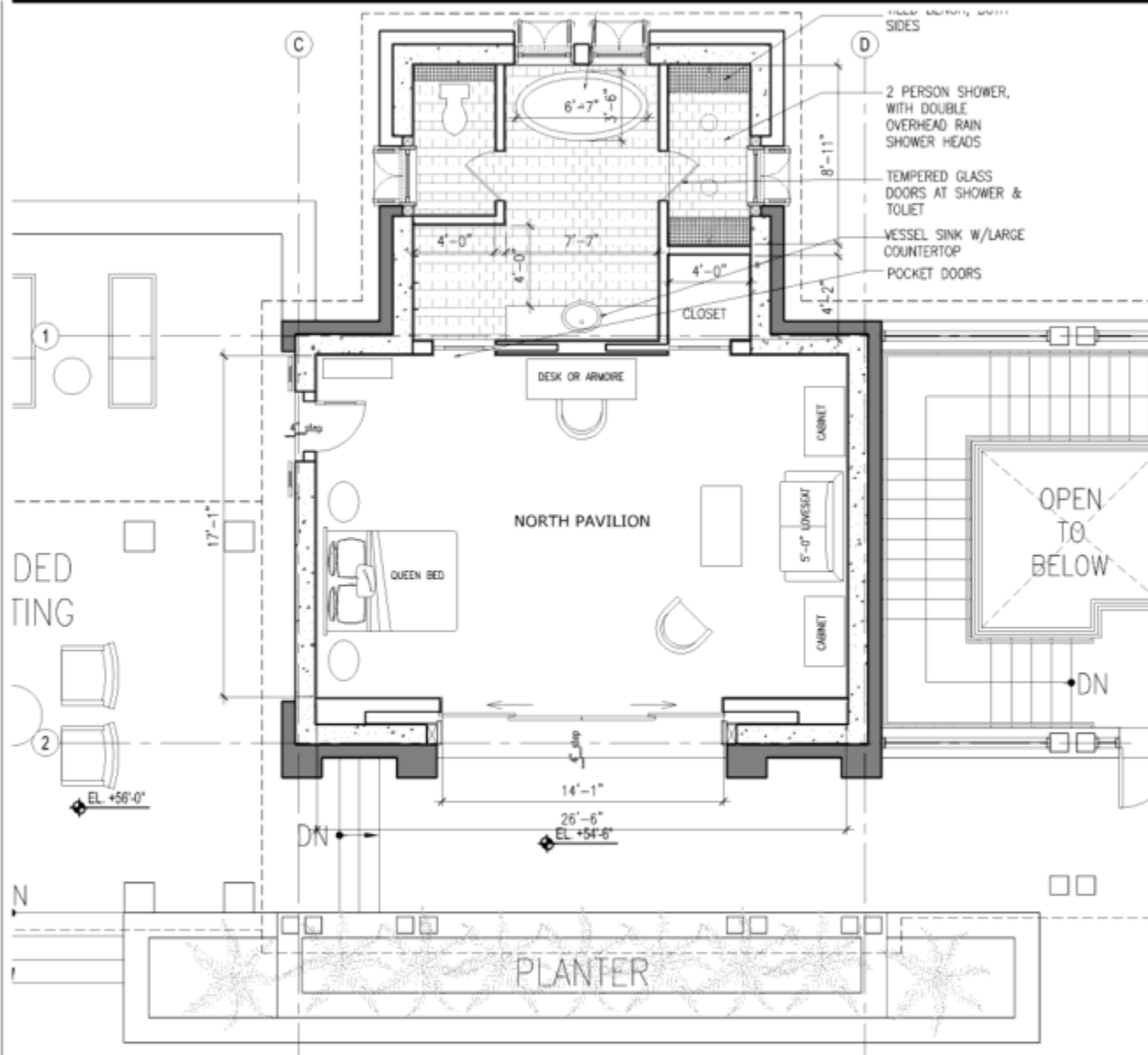
ENLARGED PLAN - NORTH PAVILION SCALE: 1/4" = 1'-0"
