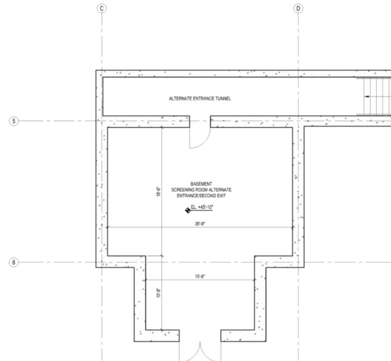
ENLARGED PLAN - SOUTH PAVILION BASEMENT SCALE: 1/4" = 1'-0"
