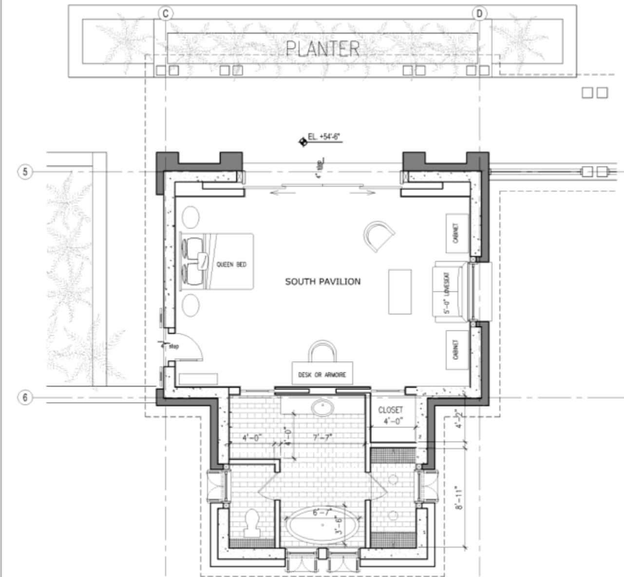
ENLARGED PLAN - SOUTH PAVILION SCALE: 1/4" = 1'-0"
