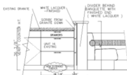
④ ELEVATION SCALE: 3/16" = 1' 0"
